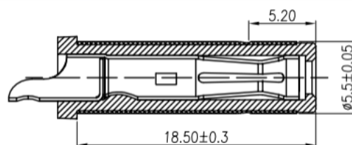
MATING PLUG
