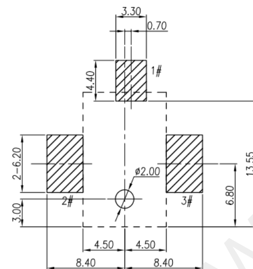
RECOMMENDED PCB LAYOUT T=1.60mm GENERAL TOLERANCE:0.05mm TOP VIEW
